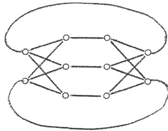
Fig. 5. G_5 = K_{2,3} \square K_2 .
