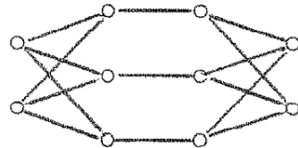
Fig. 2. The graph G_3 .
