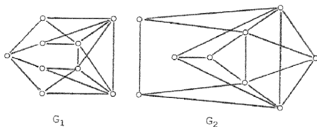
Fig. 1. Isospectral, self-complementary, Laplacian integral graphs.
