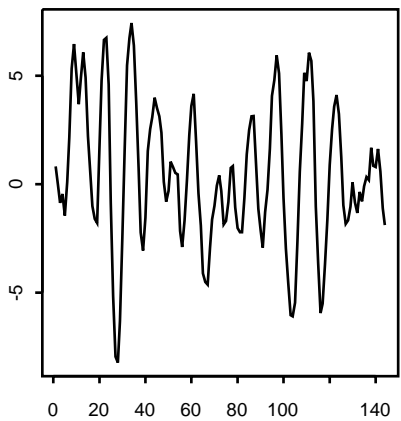
AR(2), \phi_1=1.5,\phi_2=-.75 , complex roots
