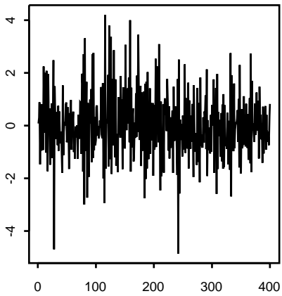
MA(2),theta_1=-.6, theta_2=.5
