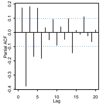
Series : x
