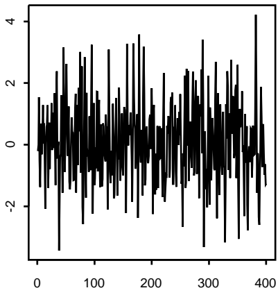
MA(2),theta_1=.6, theta_2=-.5
