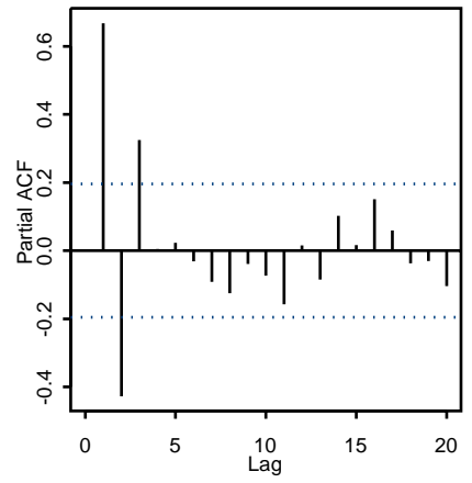
Series : x
