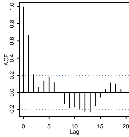
Series : x
