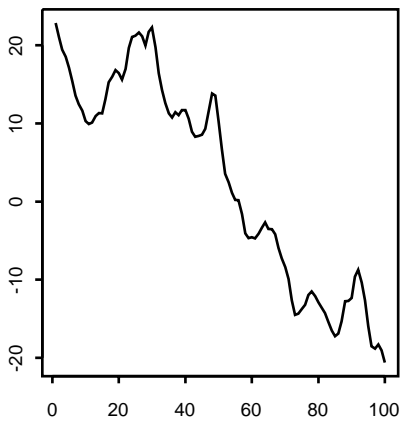
AR1MA(1,1,1),phi=.5,diff=1,theta=-.6
