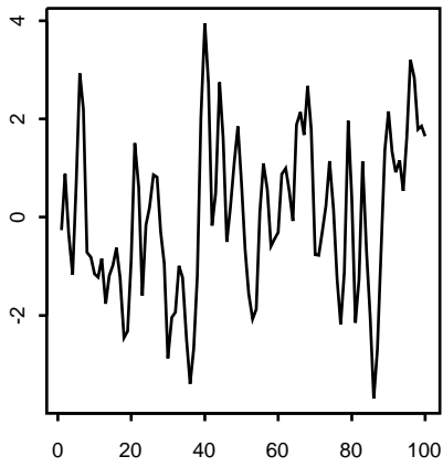
ARMA(1,1),phi=.5,theta=-.6
