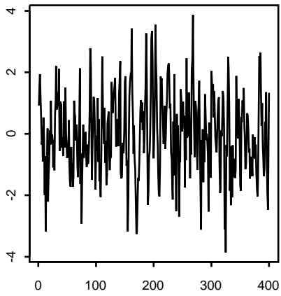
MA(2),theta_1=.6, theta_2=.5
