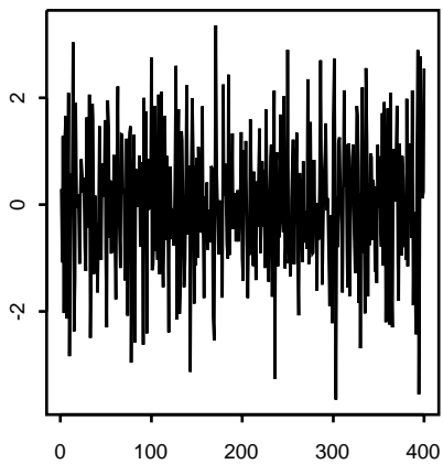
MA(2),theta_1=-.6, theta_2=-.5
